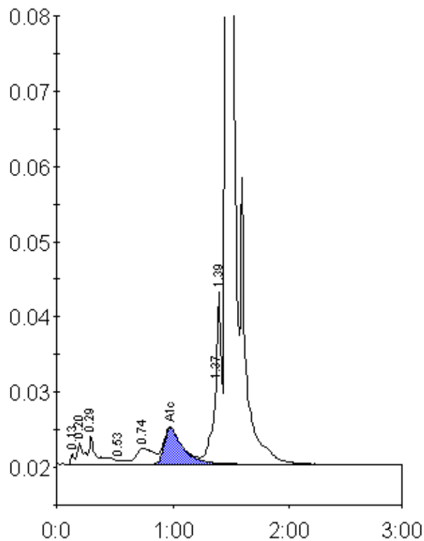
Peak table - ID: 60001140
